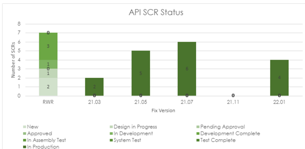
Figure 5.1.5-1 – Application Programming Interface (API) DDID Status
