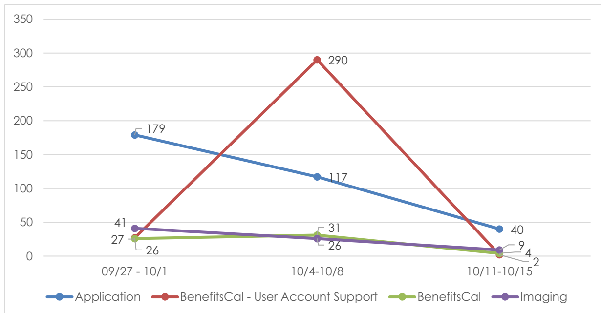
Figure 8.1.1.2 – Command Center Total Calls
